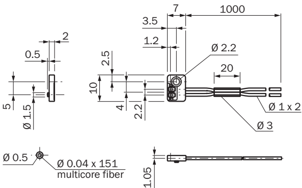
Dimensional drawing LL3-DE01
